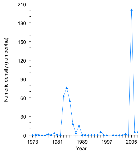
Figure 11. Numeric density of age-0 yellow perch in Lake Michigan, 1973-2007.
