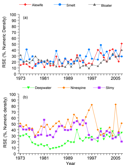
Figure 3. RSE for numeric density of Lake Michigan prey fishes, 1973-2007. Panel (a) provides estimates for adult alewife, adult rainbow smelt, and adult bloater. Panel (b) provides estimates for deepwater sculpin, slimy sculpin, and ninespine stickleback.
