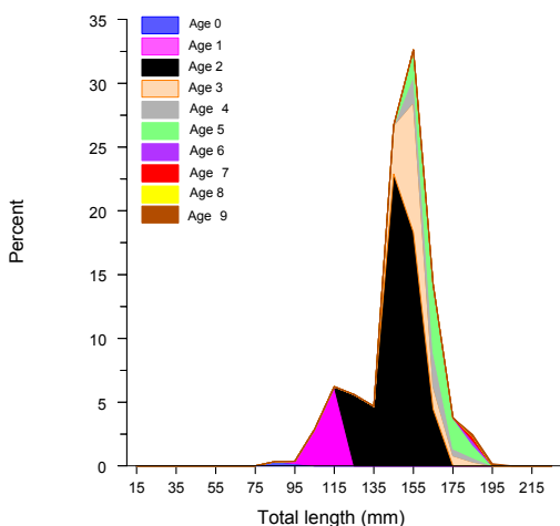
Figure 4. Age-length distribution of alewives caught in bottom trawls in Lake Michigan, 2007. Age-2 alewives belonged to the 2005 year-class.
