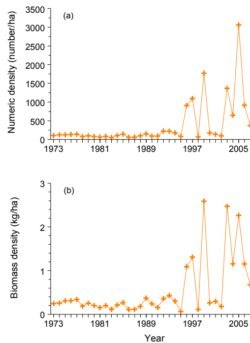
Figure 7. Density of ninespine sticklebacks as number (a) and mass (b) of fish per ha in Lake Michigan, 1973-2007.
