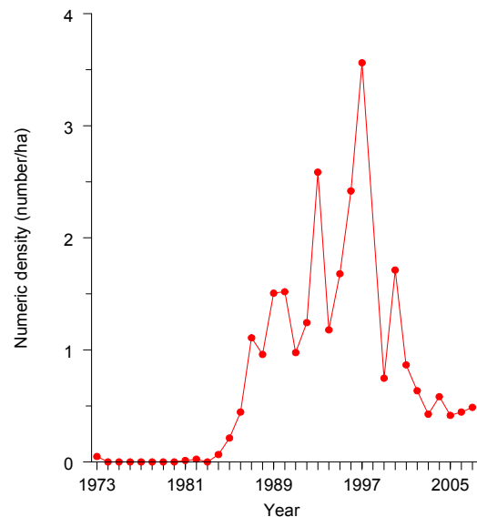
Figure 10. Numeric density of burbot in Lake Michigan, 1973-2007.
