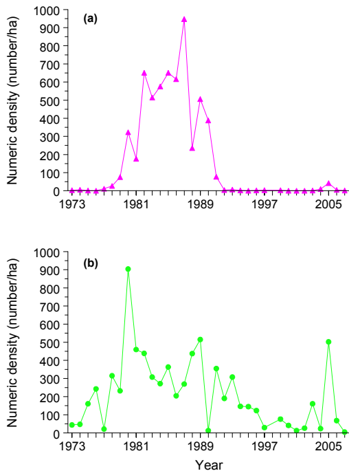
Figure 5. Numeric density of age-0 bloaters (a) and age-0 rainbow smelt (b) in Lake Michigan, 1973-2007. Time series for age-0 alewives was not included, because age-0 alewife catch was not considered a reliable indicator of alewife year-class strength (Madenjian et al. 2005a).
