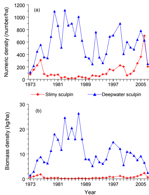
Figure 6. Density of slimy and deepwater sculpins as number (a) and mass (b) of fish per ha in Lake Michigan, 1973-2007.
