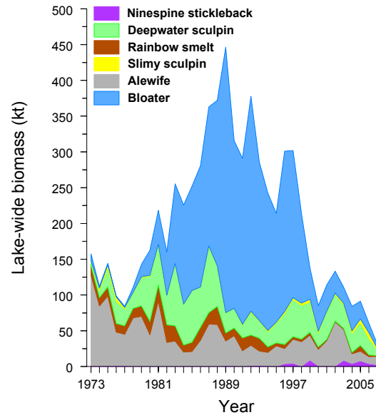
Figure 9. Estimated lake-wide biomass of prey fishes in Lake Michigan, 1973-2007, based on the bottom trawl survey.
