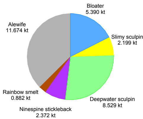
Figure 8. Estimated lake-wide biomass of prey fishes in Lake Michigan, 2007, based on the bottom trawl survey.
