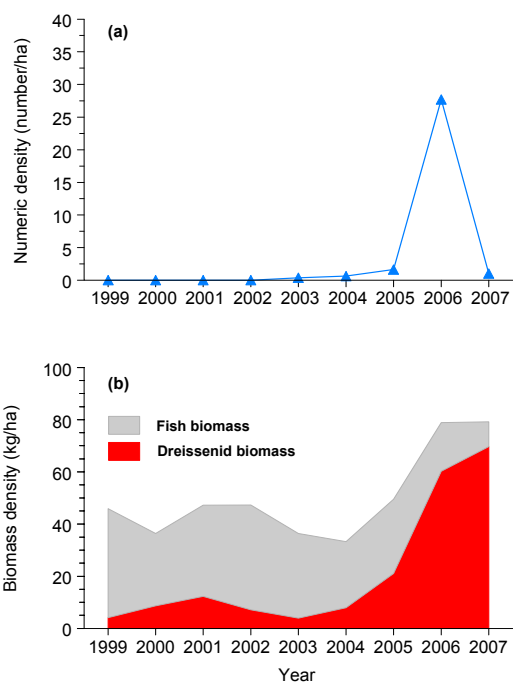
Figure 12. Estimated lake-wide numeric density of round goby (a), and total fish biomass density and dreissenid mussel biomass density (b) in Lake Michigan, 1999-2007, based on the bottom trawl survey.
