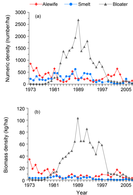
Figure 2. Density of adult alewives, rainbow smelt and bloaters as number (a) and mass (b) of fish per ha in Lake Michigan, 1973-2007.
