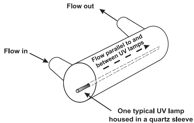
Figure 3. Wastewater flow in a quartz UV unit
