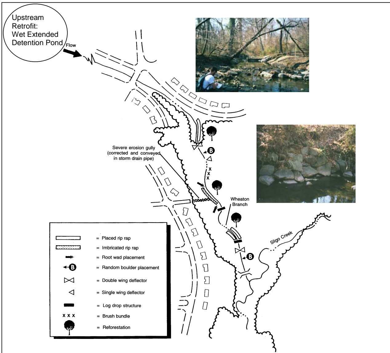
Figure 21: Example of Comprehensive Stream Restoration Approach The diagram shows the combination of stream restoration techniques employed to restore Wheaton Branch in Montgomery County, Maryland. A key element of the project was the construction of an upstream storage retrofit used to remove pollutants and control hydrology, along with riparian reforestation and restocking of native fish species. The restoration project was built in the late 1980s, and resulted in improved fish and aquatic diversity in this formerly non-supporting stream.
