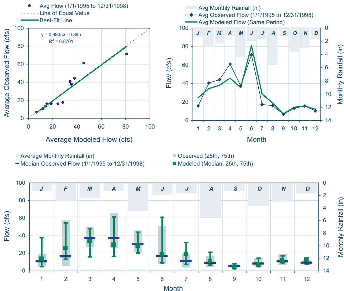
Figure 8-3. Sample Calibration Tests for Hydrologic Simulation
